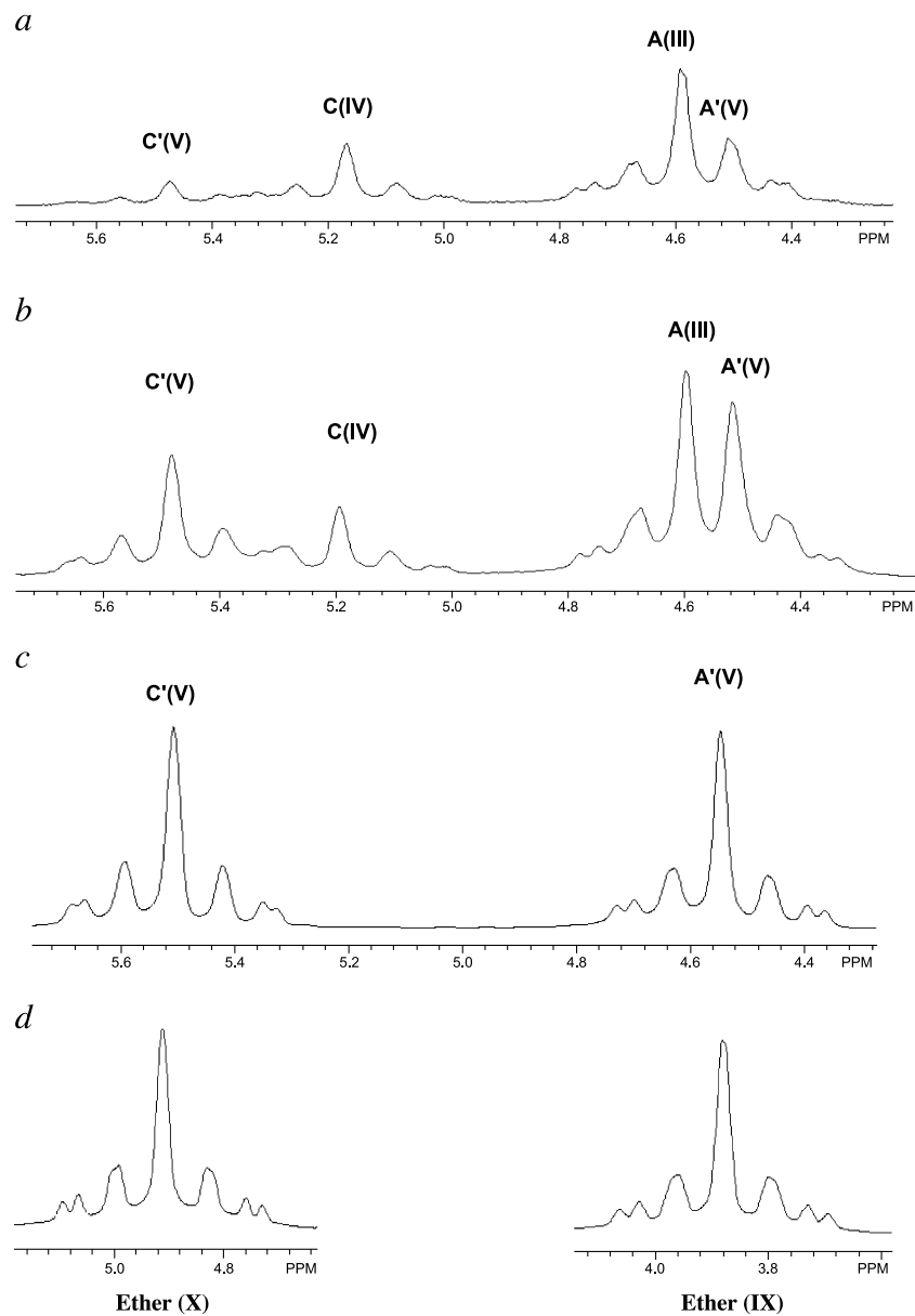
FIGURE 1 Fragments of ^{19}\text{F} NMR spectra of the reaction mixtures (Scheme 1) that correspond to [\beta], [\beta]' -fluorine atoms of pyridyl rings A, C, A', and C' of (III), (IV), and (V). The spectra are registered after 0.75 (a), 3 (b), and 16 (c, final) h after the beginning of the reaction; (d), fragments of ^{19}\text{F} NMR spectra of the reaction mixtures containing [\beta], [\beta]' -fluorine atoms of pyridyl rings of ethers (VII) and (VIII).
