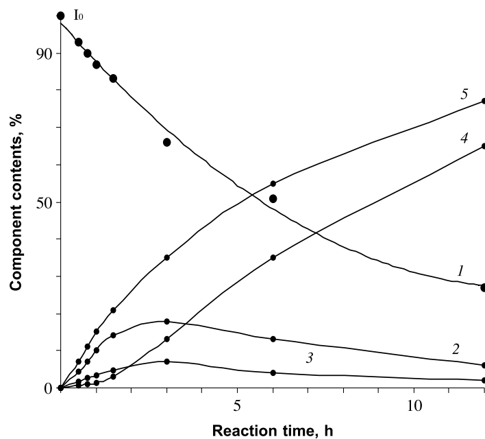
FIGURE 2 Kinetic curves of arylation of thymidine with pentafluoropyridine. The relative content of components of the reaction mixture is considered as (I_i/I_0) 100\% , where I_i and I_0 are the integral intensities of fluorine resonances of the reaction components and the initial pentafluoropyridine, respectively: 1, substrate (I); 2, intermediate (III); 3, intermediate (IV); 4, diether (V); 5, the overall content of ethers (III)–(V) and triethylamine hydrofluoride (VI).
